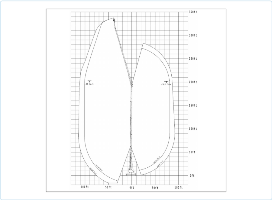
WORKING ENVELOPE
