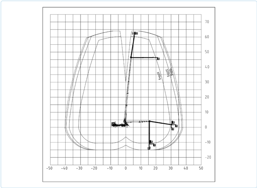
WORKING ENVELOPE
