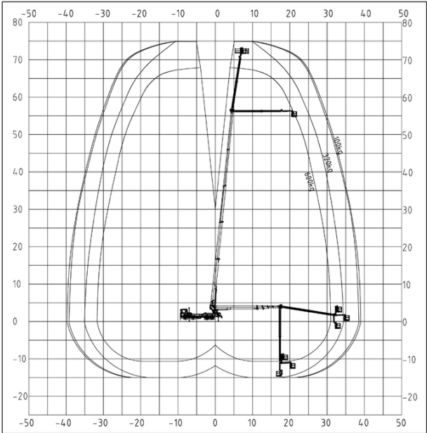
WORKING ENVELOPE
