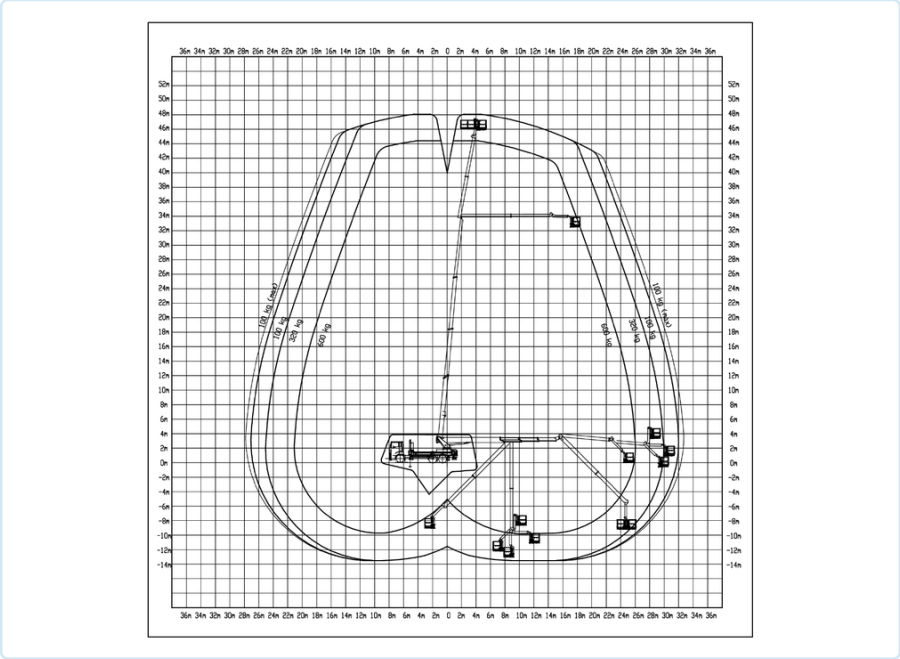
WORKING ENVELOPE
