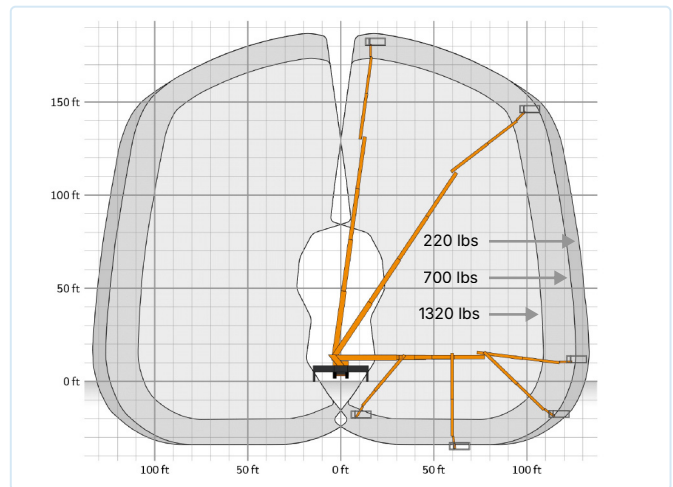
WORKING ENVELOPE
